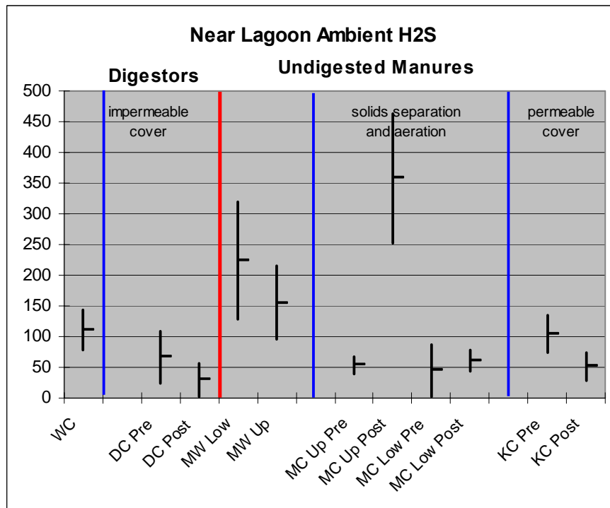
Figure I Near Lagoon Hydrogen Sulfide Concentrations
