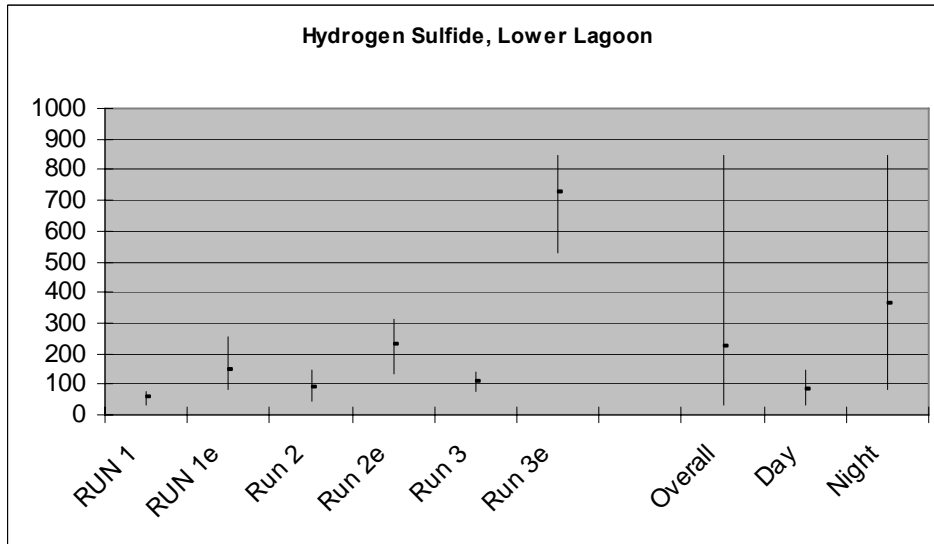
Figure 6.3 Hydrogen Sulfide, Lower Lagoon (Manitowoc County)
