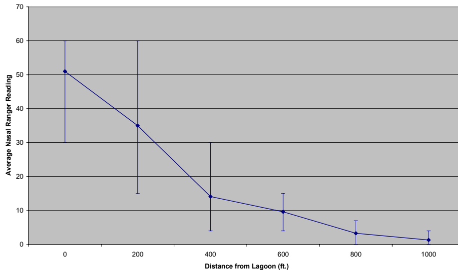
Figure 6.8 Average Nasal Ranger™ Reading at 200 ft Intervals Baseline Manure Storage Lagoon (Manitowoc County)
