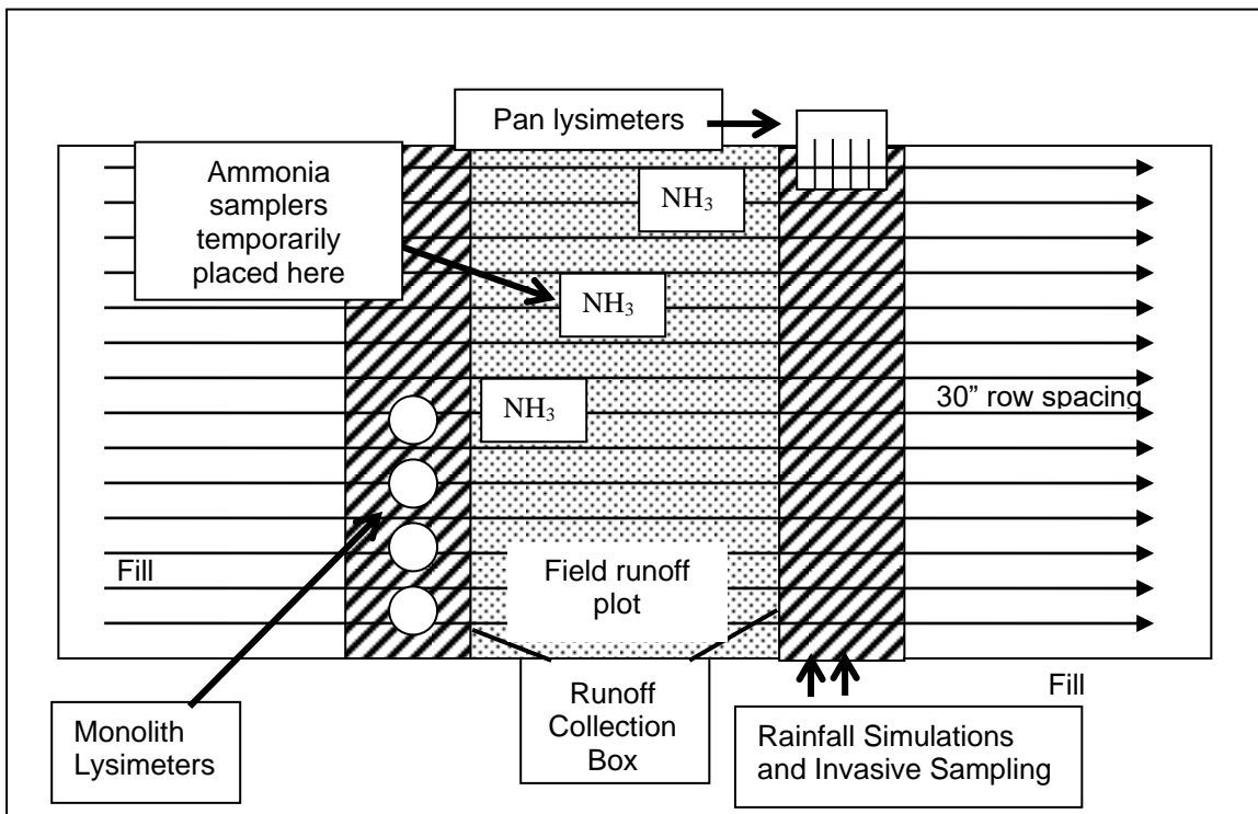
Figure 2. Layout of individual field plots.
