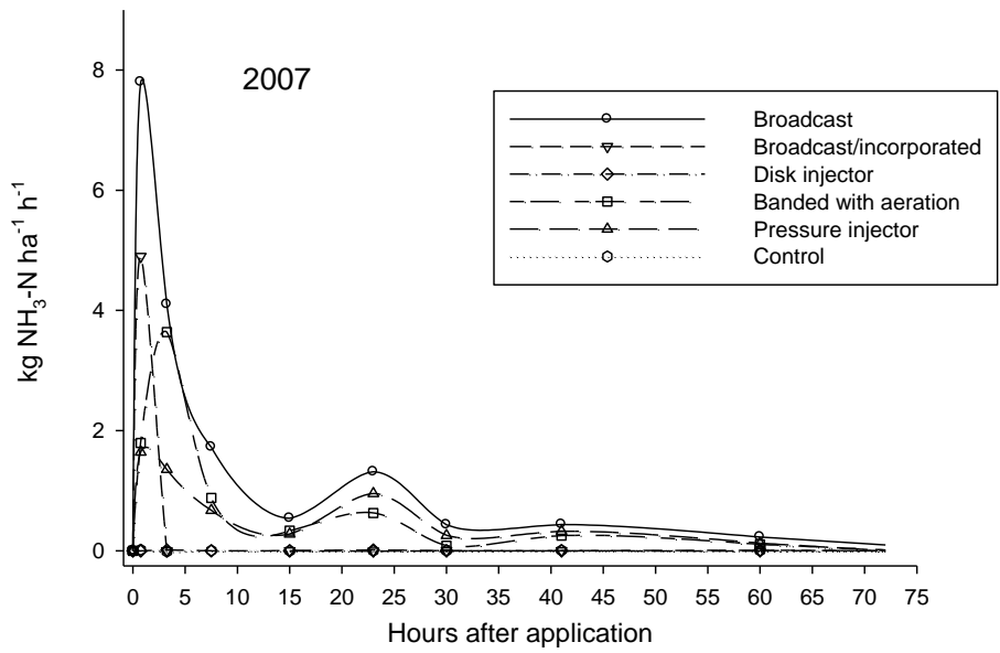
Figure 3. Ammonia-N emission rates over the 72-h observation period immediately following manure application by various methods in 2006 and 2007.
