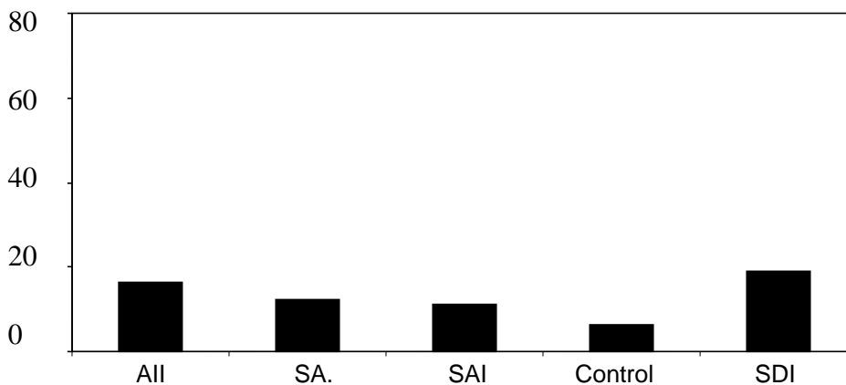
Figure 10. 2005 mean particulate phosphorus concentrations (mg/plot) in runoff from small plots (2 x 2 m) for control, surface application (SA), surface application incorporation (SAI), aeration infiltration injection (AII), and shallow disk injection (SDI)
