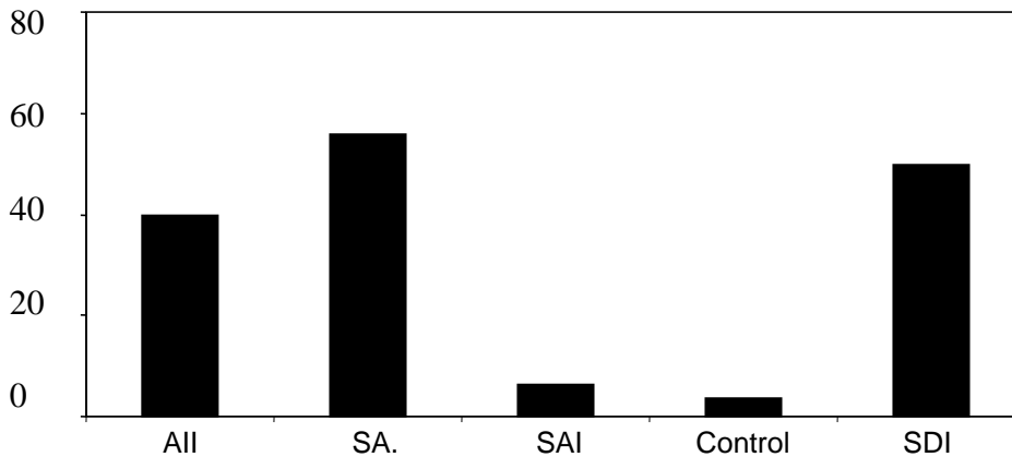
Figure 9. 2005 mean dissolved phosphorus concentrations (mg/plot) in runoff from small plots (2 x 2 m) for control, surface application (SA), surface application incorporation (SAI), aeration infiltration injection (AII), shallow disk injection (SDI) and pressure injection (PI)
