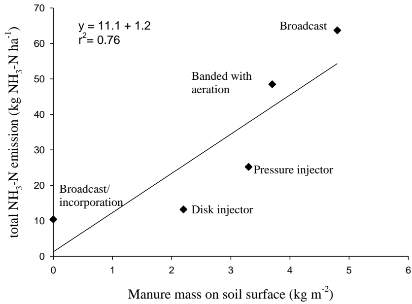
Figure 4. The relationship between total ammonia emissions and manure remaining on the soil surface following manure application by five methods.
