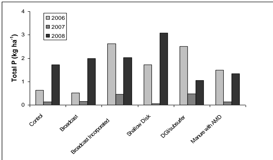
Figure 13. Total phosphorus loads (kg ha -1 ) in leachate for the different low disturbance manure injectors at Princess Anne, MD.
