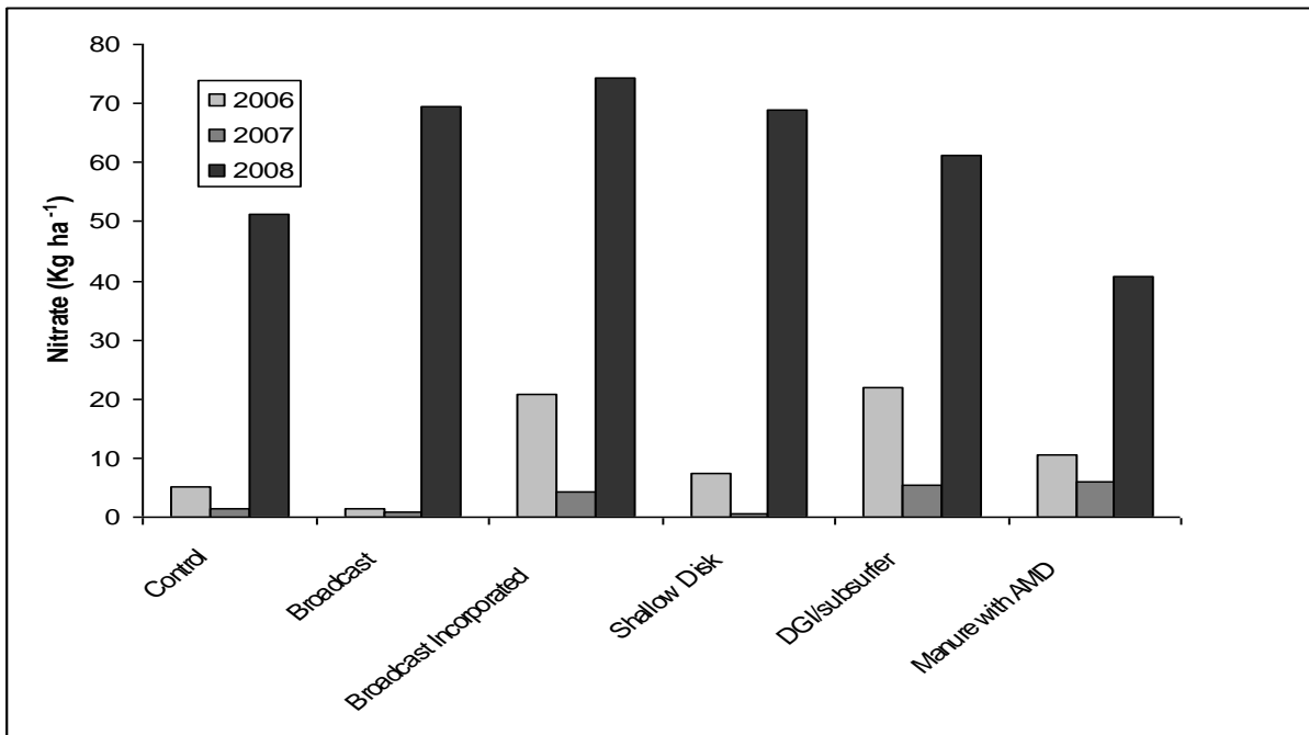
Figure 14. Nitrate nitrogen loads ( \text{kg ha}^{-1} ) in leachate for the different low disturbance manure injectors at Princess Anne, MD.
